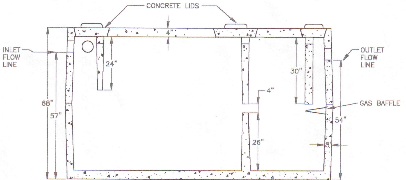
CUT AWAY SIDE VIEW
