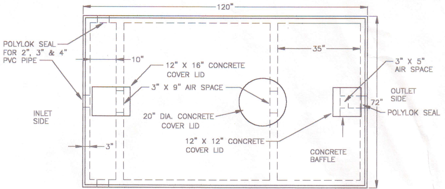
TOP VIEW
