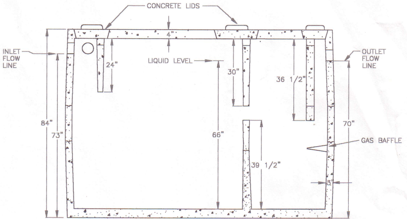
CUT AWAY SIDE VIEW
