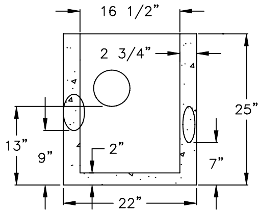
CUT AWAY SIDE VIEW KNOCKOUTS AT 7", 9", 13", AND 15" HEIGHTS
