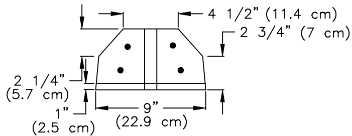
ENLARGED END VIEW (SHOWING REINFORCEMENT)
